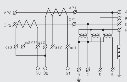
2 大变比接线图 Big ratio connection drawing
