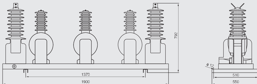
组合互感器接线图: Combined transformer connection drawing
