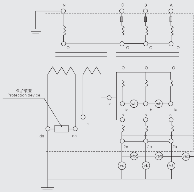
Double measurement wiring elementary diagram
